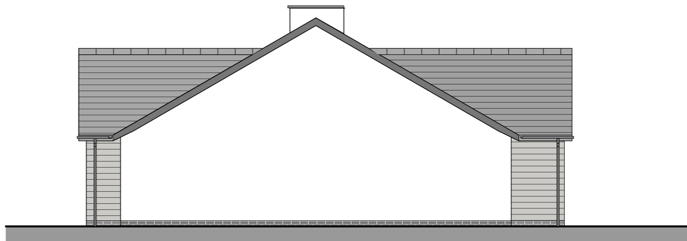
WEST ELEVATION
