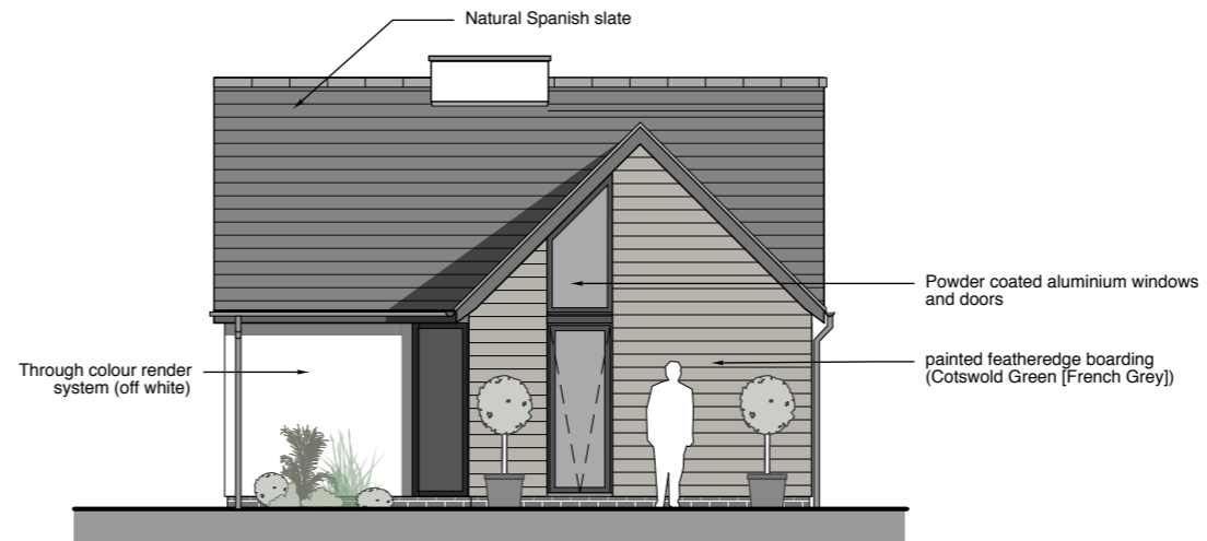
NORTH ELEVATION
